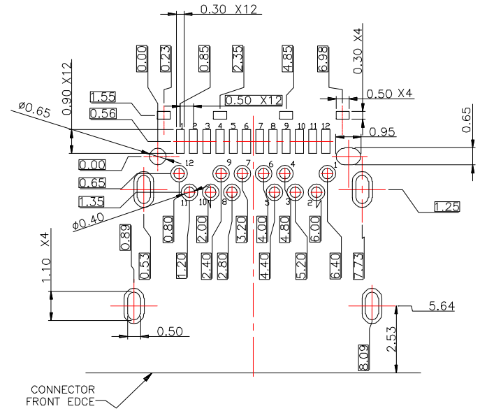
P.C.B LAYOUT MOUNTING PATTERN
