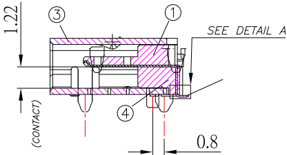
SECTION B-B SCALE 4:1
