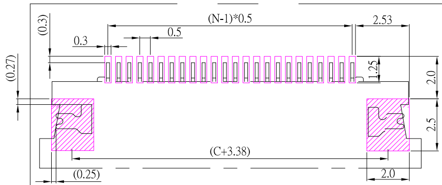
PCB LAYOUT
