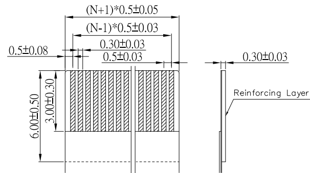
APPLICABLE FPC/FFC
