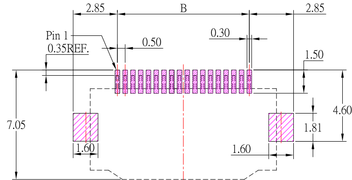
PCB LAYOUT
