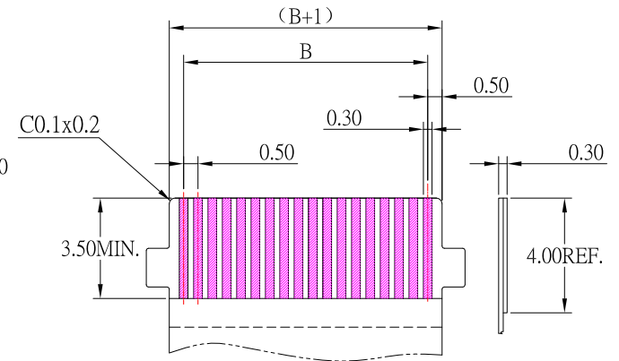
APPLICABLE FPC/FFC
