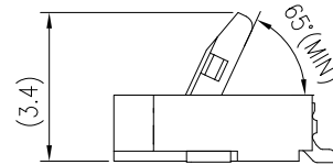
COVER OPEN STATE
