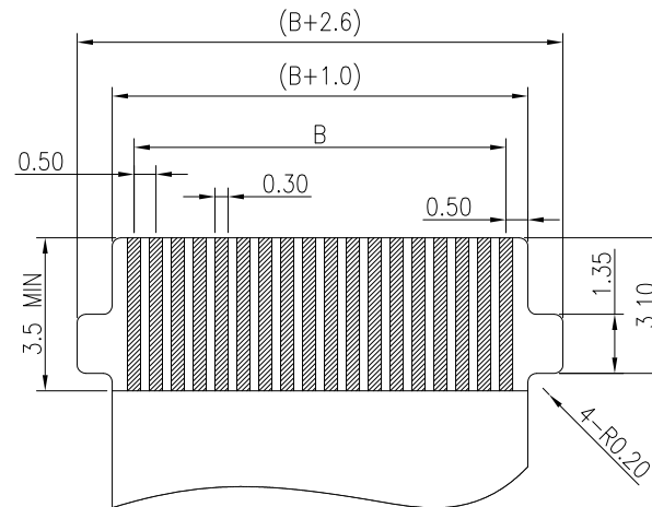
APPLICABLE FPC/FFC
