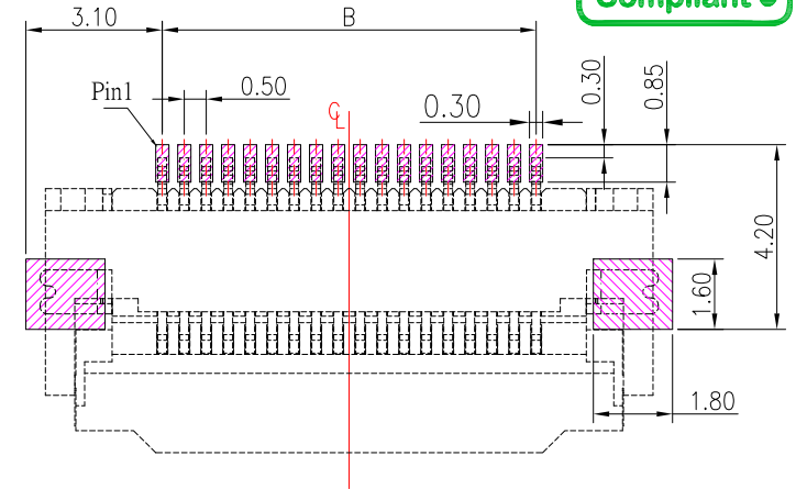
PCB LAYOUT
