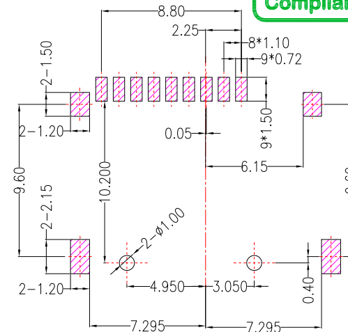
PCB LAYOYT
