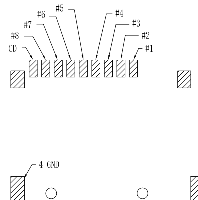
PIN ASSIGNMENT
